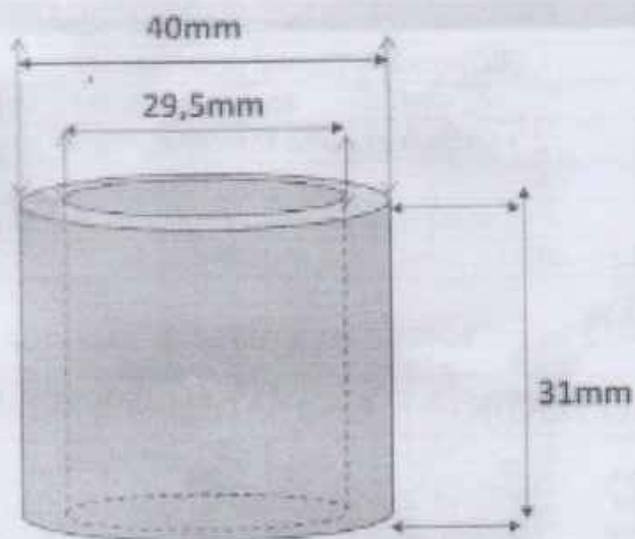
Female Bushing Stirrer
