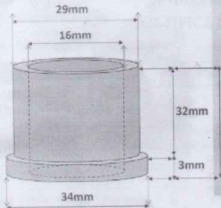
Male Bushing Stirrer
