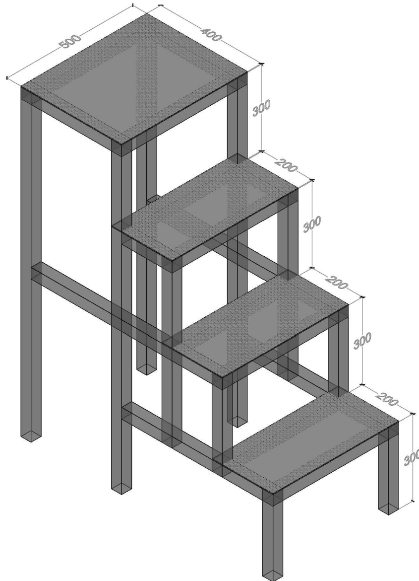
STAIRCASE CIP SYSTEM 8B
