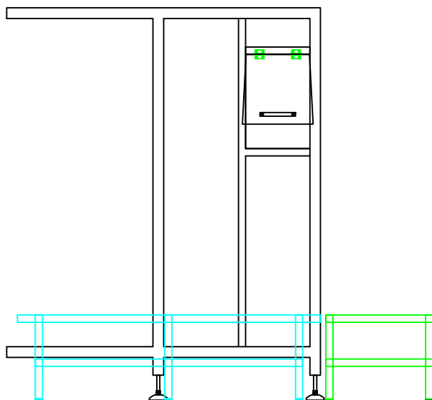
STEP PLATFORM - PORTS TRANSFER AREA (FFS UNIT 8B)
