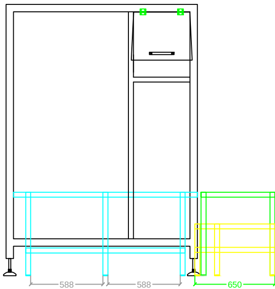
STEP PLATFORM - CAPS TRANSFER AREA (FFS UNIT 8B)
