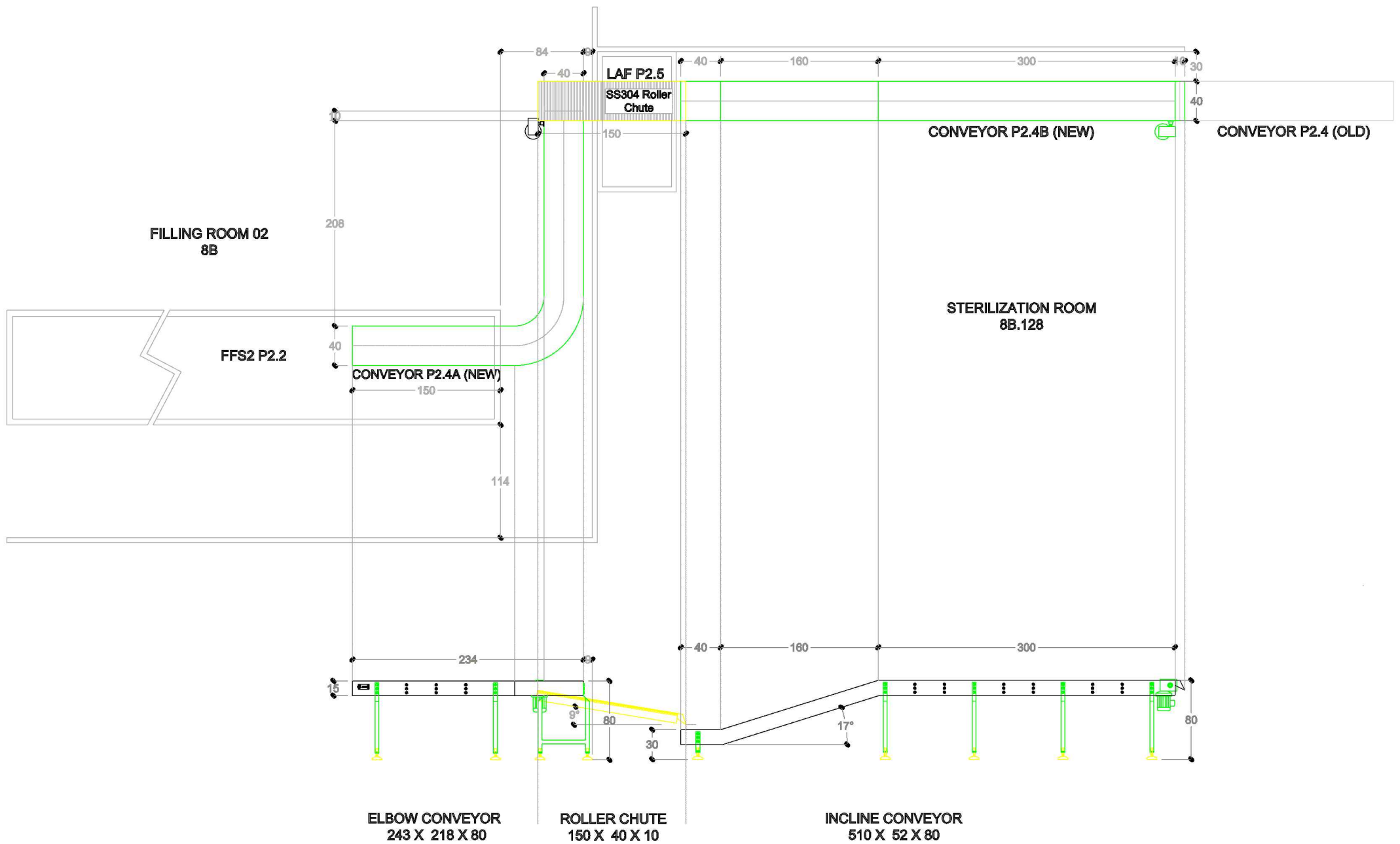
ELBOW CONVEYOR , ROLLER CHUTE & INCLINE CONVEYOR LINE 2 UNIT 8B (AFTER FFS2)
