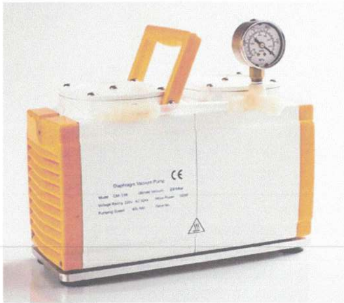
Lampiran 1. Gambar Diaphragm Vacuum Pump ( Oil free )
